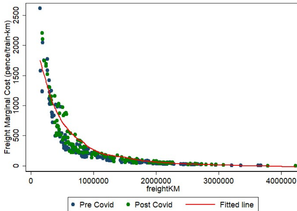
Figure 6.5: Freight marginal costs by traffic
