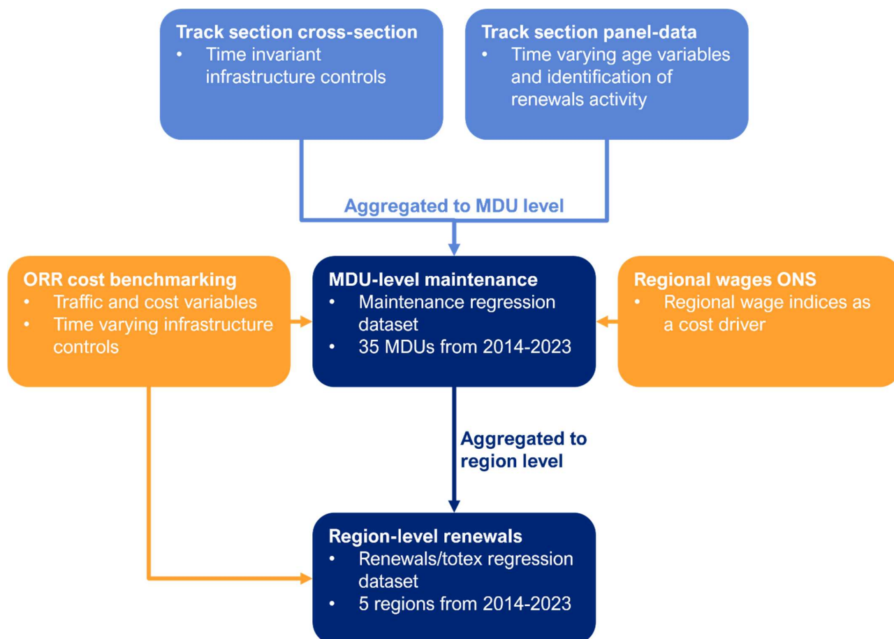
Figure 4.1: Constructing datasets for regression analysis
